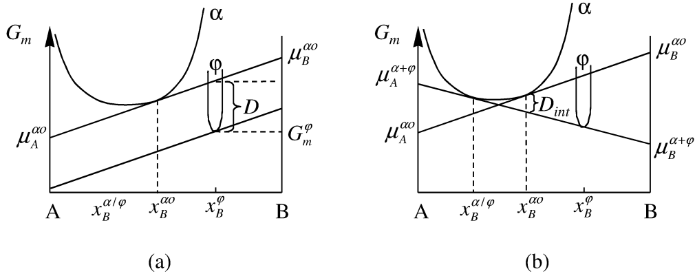
Figure 1.7: (a) Construction to find the initial driving force D for precipitating a binary \phi phase from a solution phase of an initial composition x_B^{\alpha o} . (b) Diagram showing the final composition, x_B^{\alpha/\phi} , of the parent phase at the \alpha + \phi equilibrium. D_{int} is the integrated driving force for the complete precipitation process.
